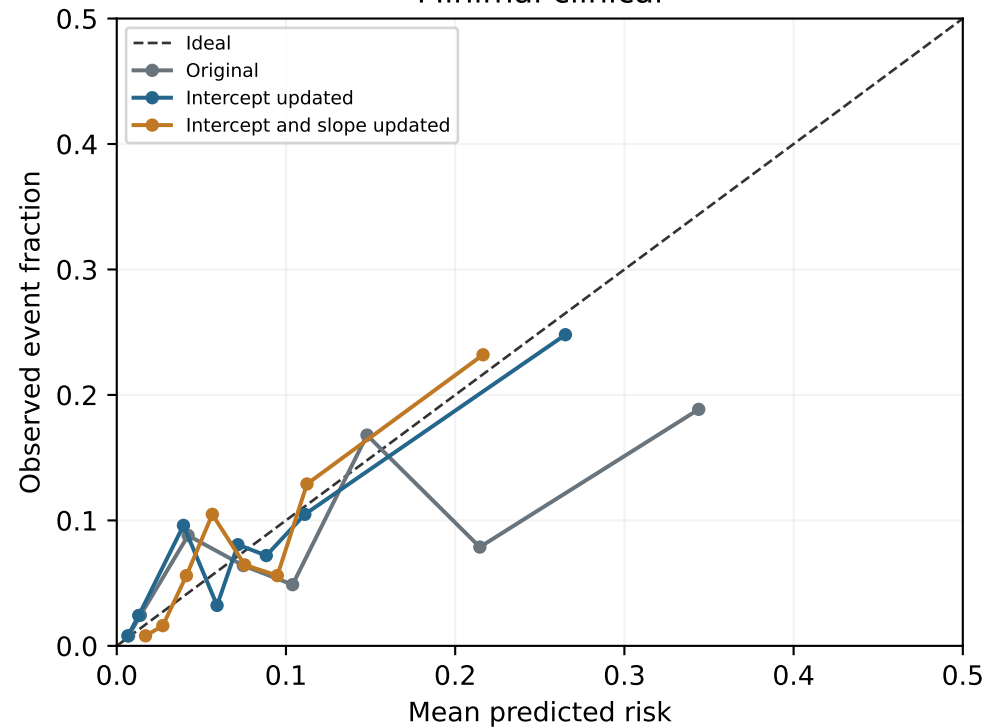
Minimal clinical
