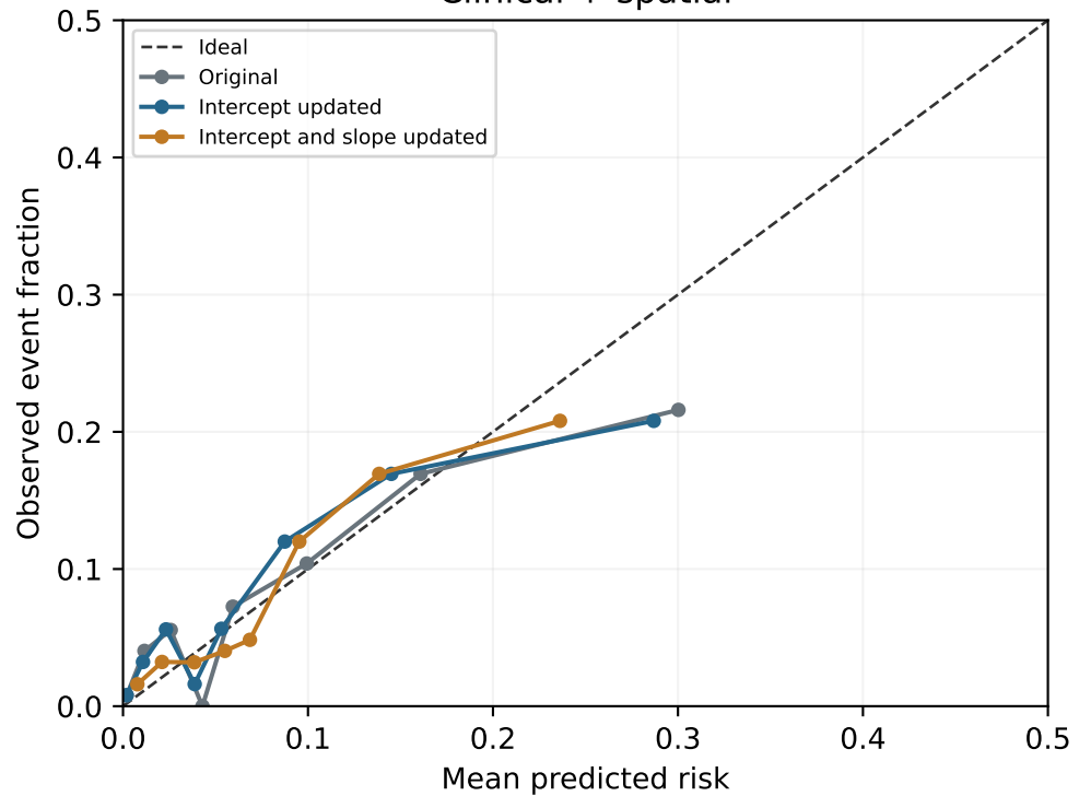
Clinical + spatial
