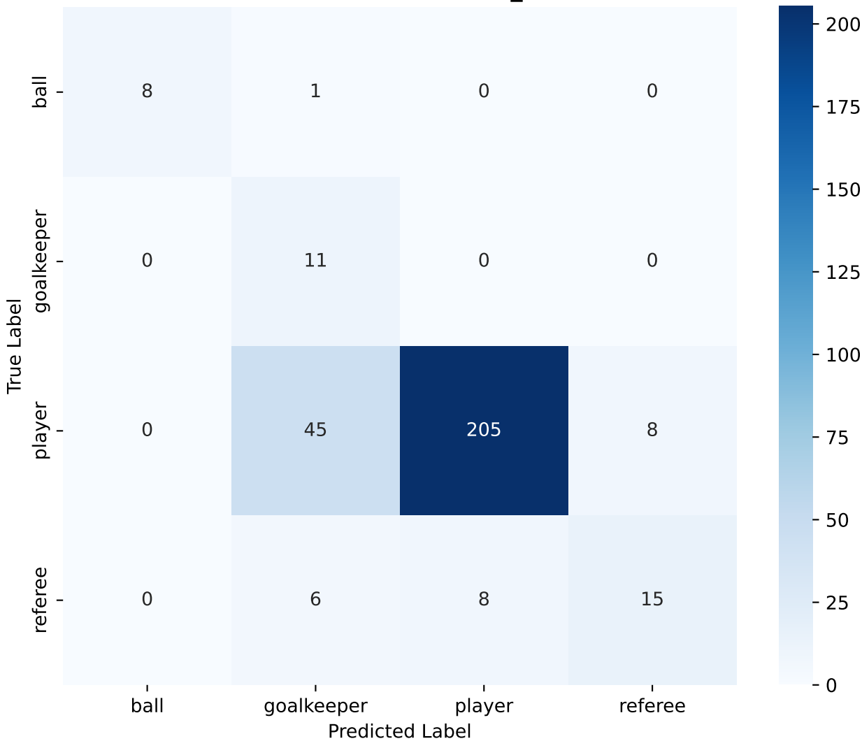
Confusion Matrix — Custom_CNN (test)
