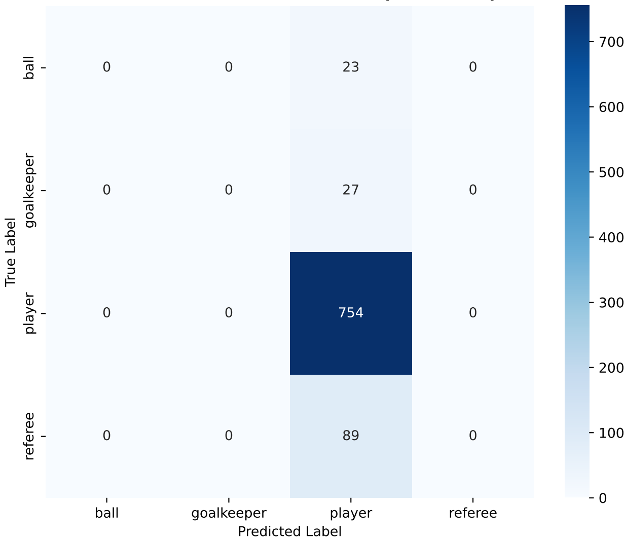
Confusion Matrix — ResNet50 (validation)
