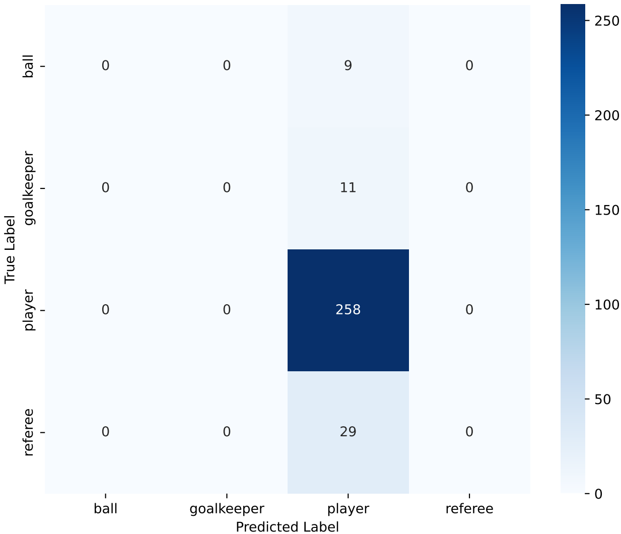
Confusion Matrix — ResNet50 (test)
