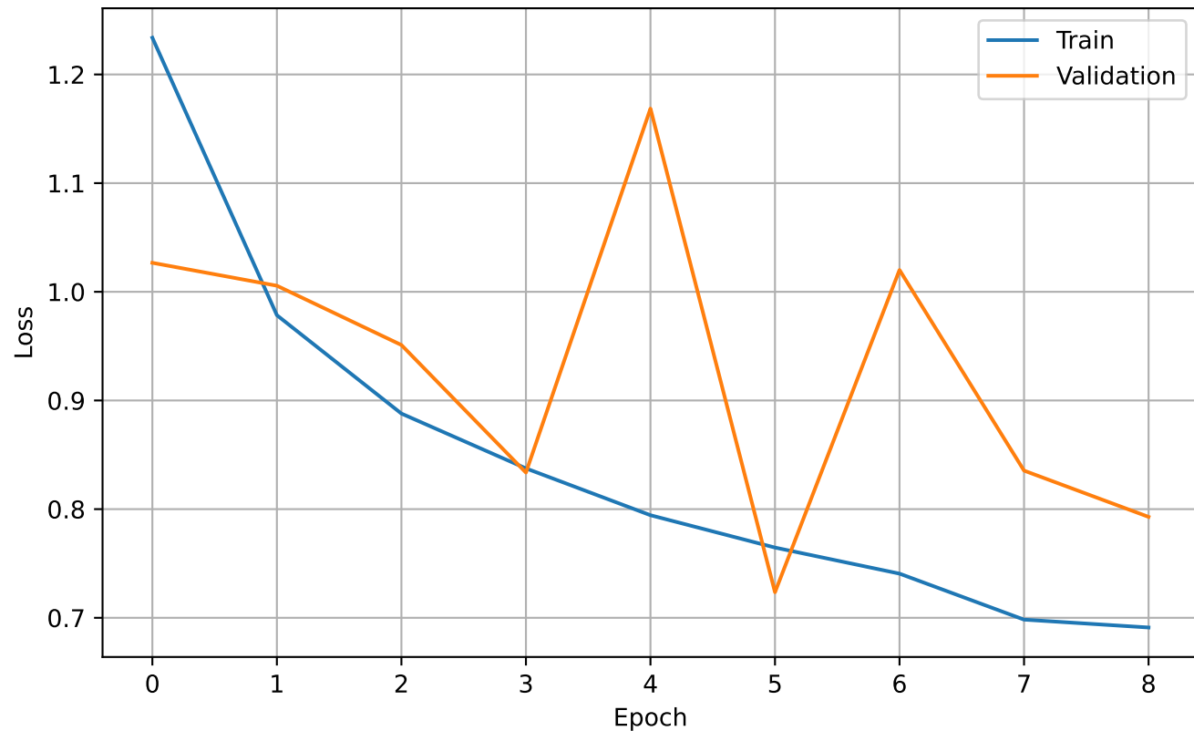
ResNet50 — Loss
