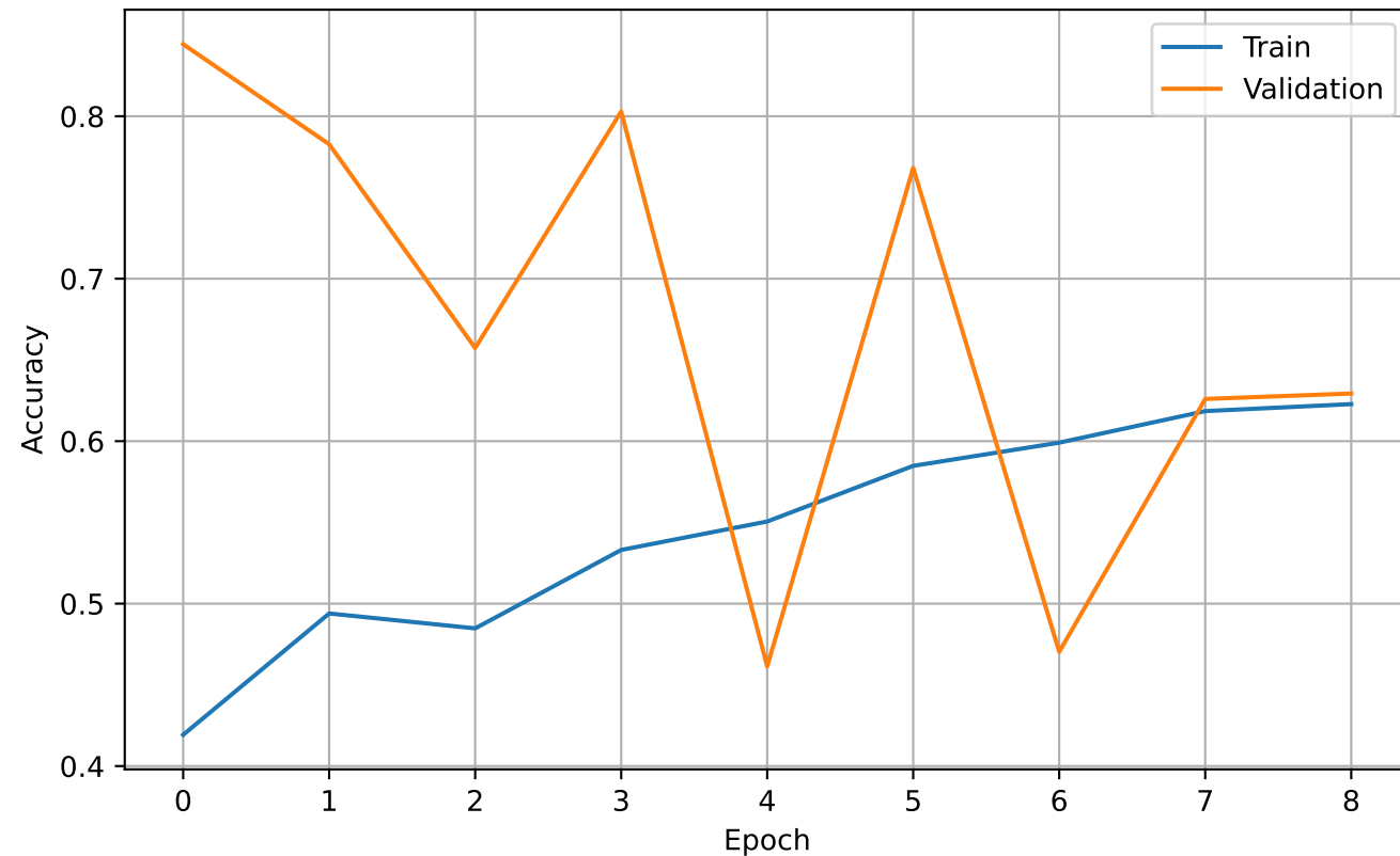
ResNet50 — Accuracy
