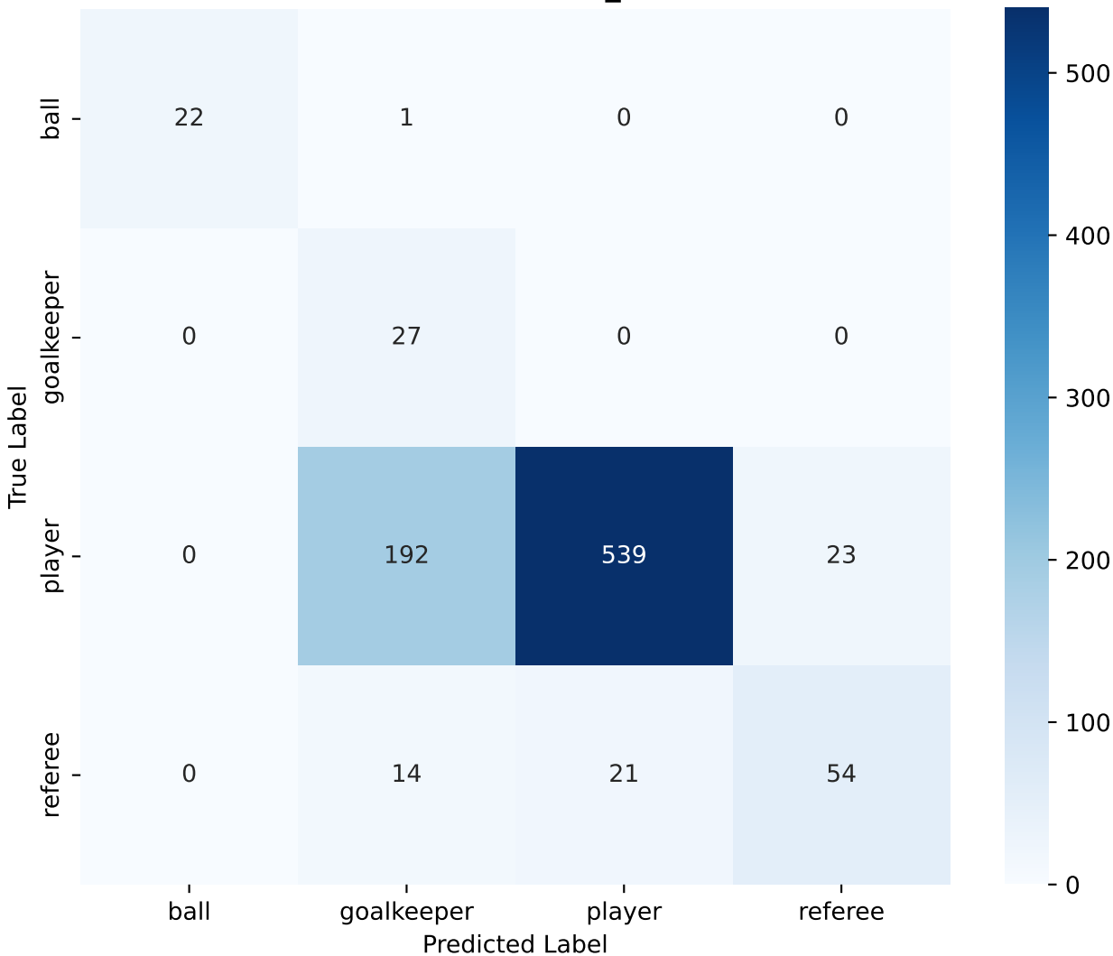
Confusion Matrix — Custom_CNN (validation)
