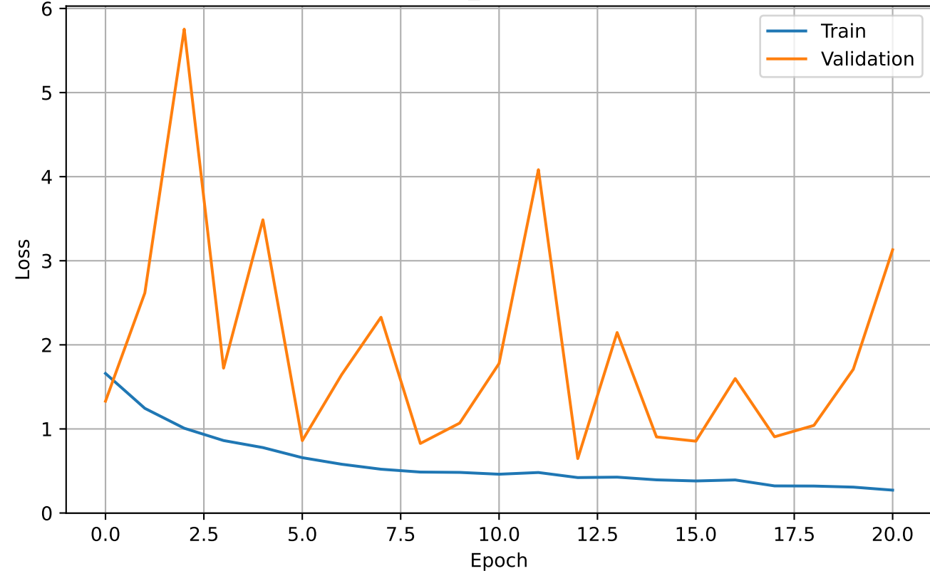
Custom_CNN — Loss
