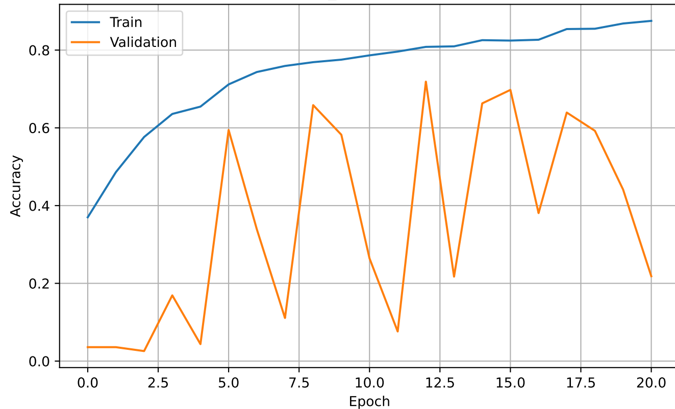
Custom_CNN — Accuracy
