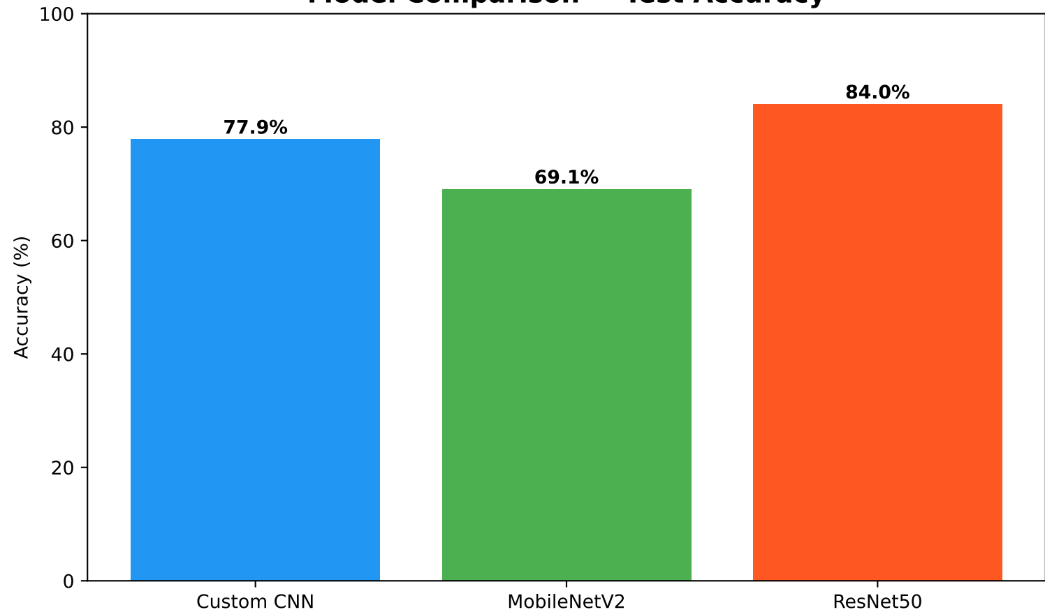
Model Comparison — Test Accuracy
