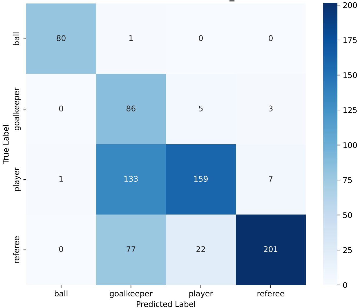
Confusion Matrix — Custom_CNN
