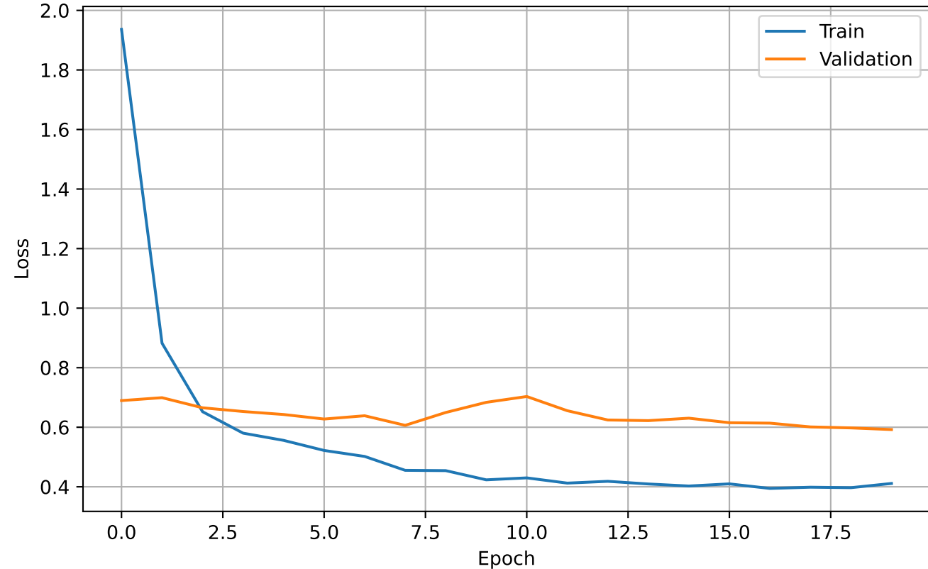
MobileNetV2 — Loss
