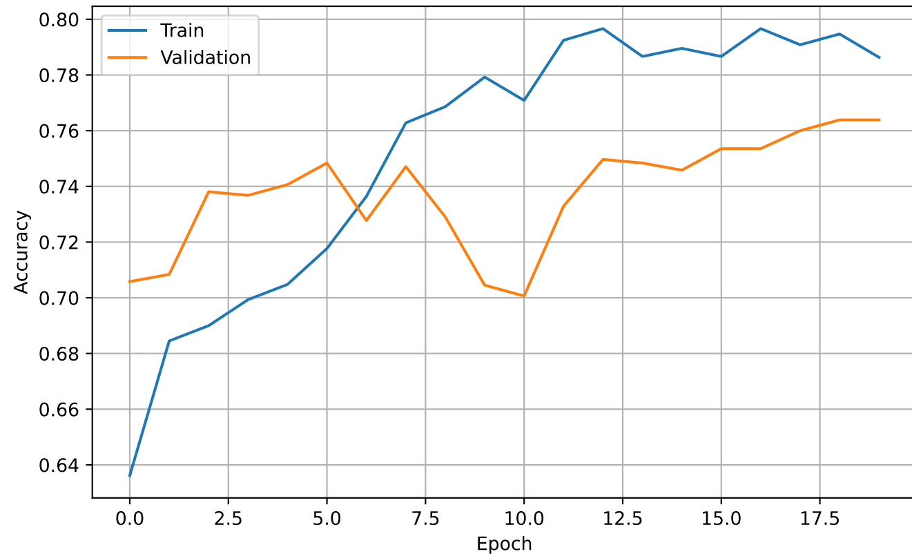
MobileNetV2 — Accuracy
