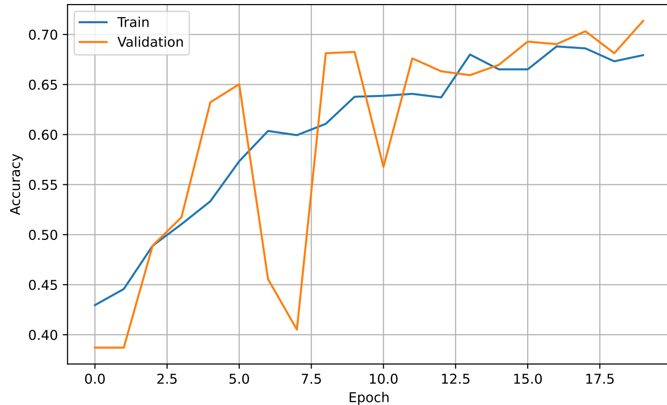
ResNet50 — Accuracy
