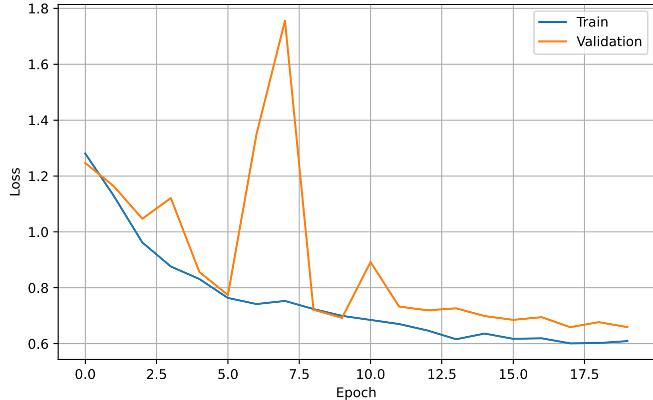
ResNet50 — Loss
