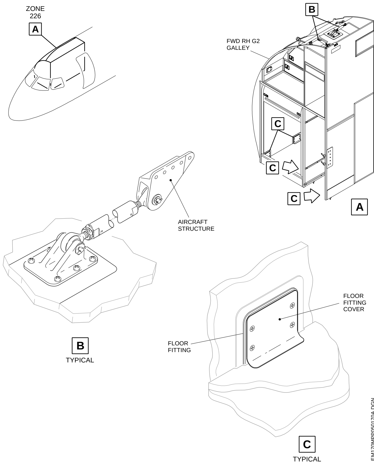
EFFECTIVITY: ALL Galley Attachments - Inspection Figure 610 - Sheet 2
