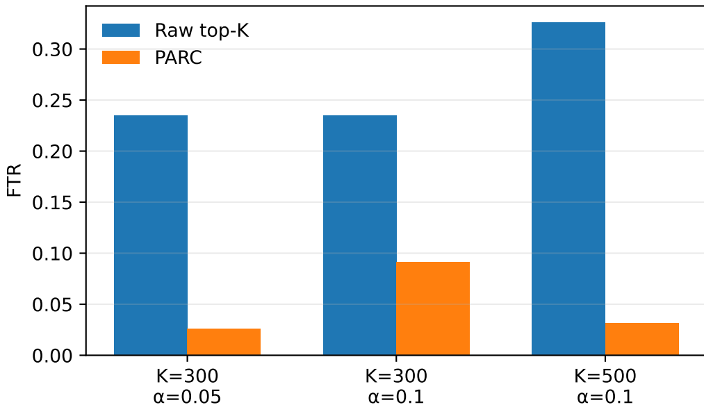
Materials raw top-K vs PARC
