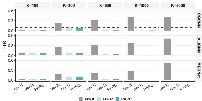
Model-budget FTR frontier
