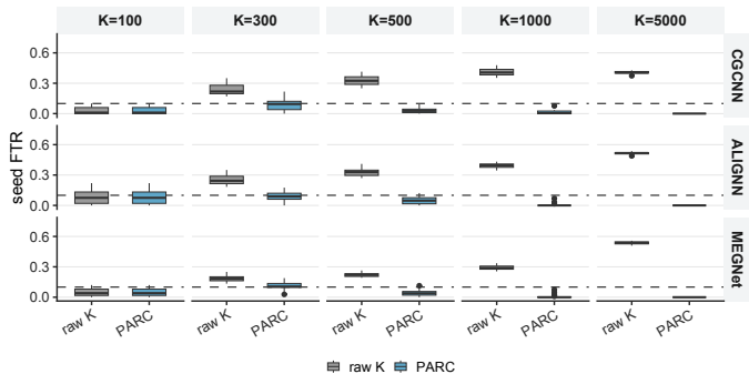
Seed-level FTR distributions
