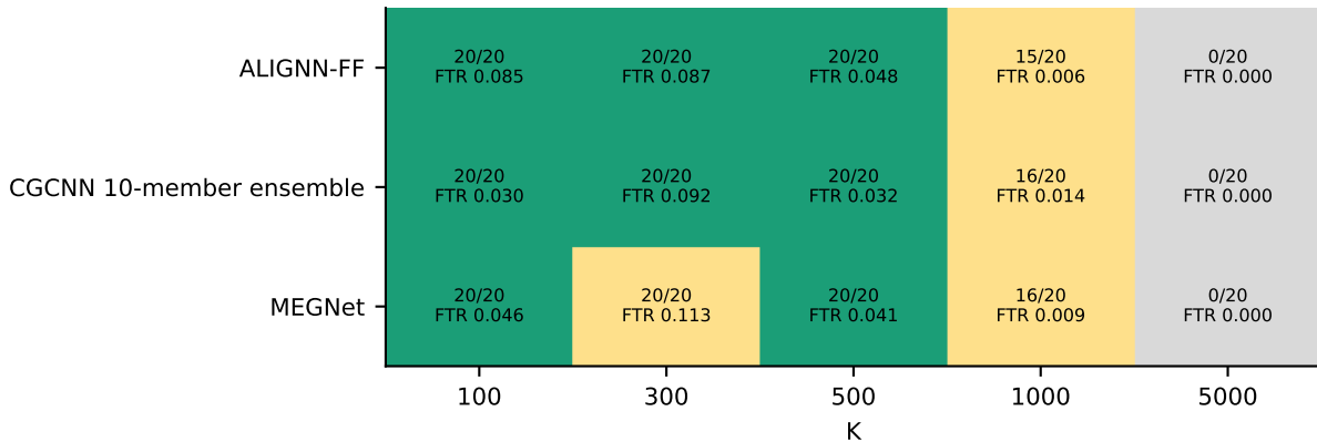
Materials release/refusal frontier, \alpha=0.10
