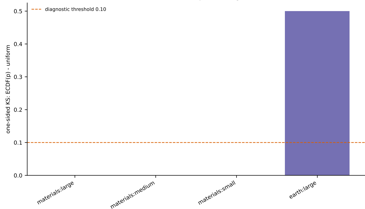
Block-size stratified p-value diagnostic
