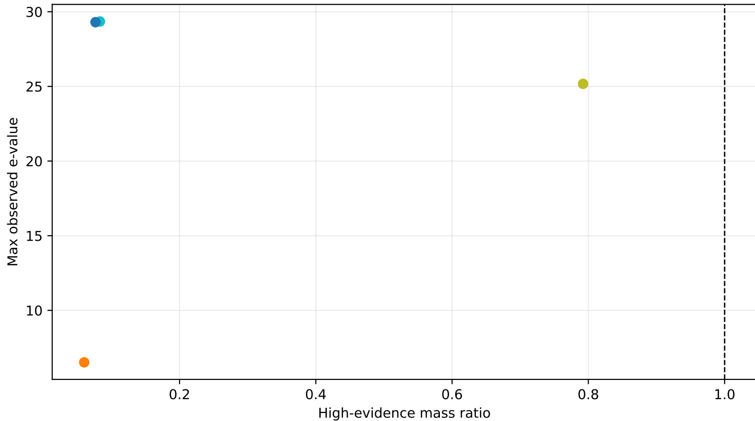
Safe-refusal evidence diagnostics
