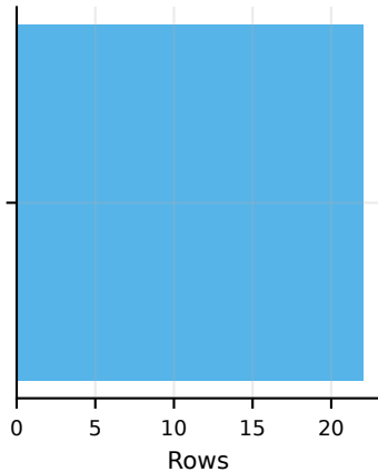
Refusal reasons
