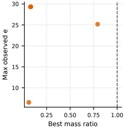
Refusal evidence
