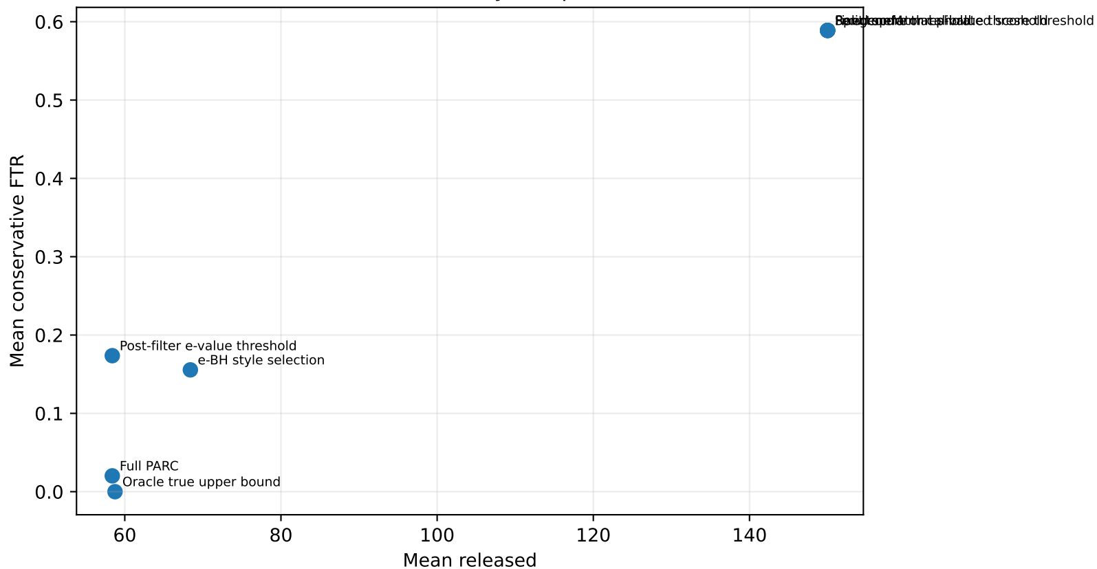
Baseline risk-utility comparison
