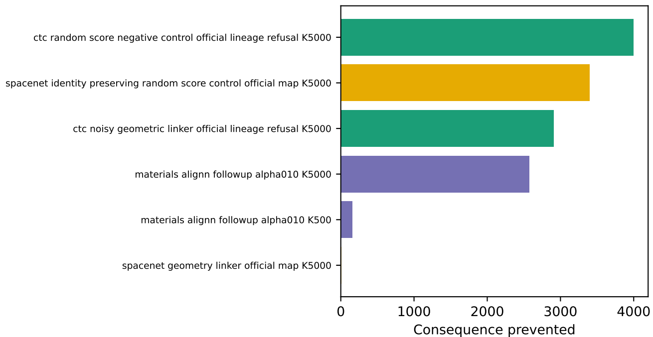
Guardrail cards
