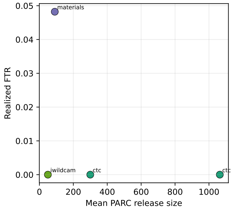
Release cards
