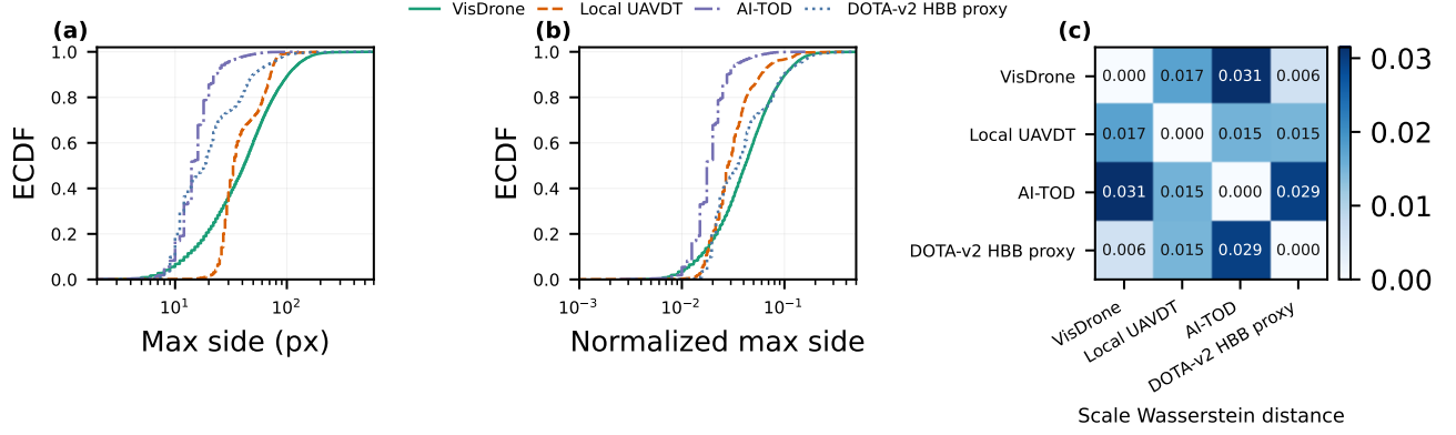
Fig. 1. Structural audit: (a) absolute horizontal-box support, (b) normalized support, and (c) equal-box-weight empirical 1-Wasserstein distances on normalized max side. DOTA-v2 is an axis-aligned horizontal-box (HBB) proxy derived from quadrilaterals and is structural-only; its distances are representation-conditioned rather than directly comparable to native horizontal-box sources.
