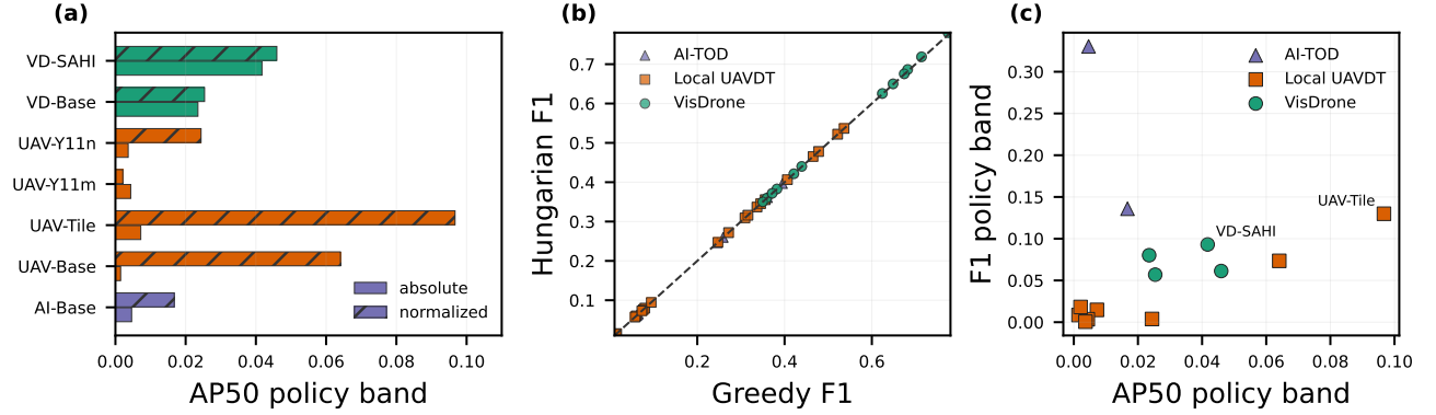
Fig. 2. Primary-grid rule and matching sensitivity: (a) AP_{50} bands over \Pi = \{\text{include-all}, \text{exclude/source-ignore-off}, \text{exclude/source-ignore-on}\} at the two headline scale rules (solid: absolute; hatched: normalized; VD=VisDrone, UAV=local UAVDT, AI=AI-TOD; Base=baseline, Tile=tiling, SAHI=slicing-aided inference, Y11n/Y11m=YOLO11 variants), (b) score-ordered greedy versus threshold-first Hungarian F_1 at confidence .25 and IoU .25/.50, and (c) AP_{50}/F_1 primary-grid policy-band relation. Circle/square/triangle markers denote VisDrone/local UAVDT/AI-TOD, respectively; points use source-consistent coverage.
