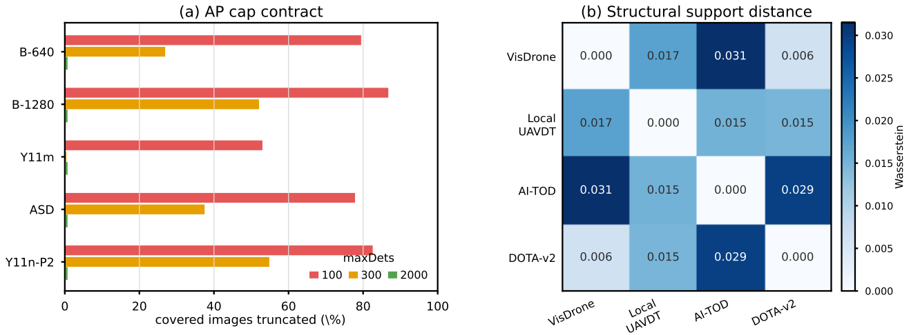
Fig. S3. Ancillary controls. (a) Fraction of the 548 covered VisDrone images whose mapped vehicle predictions exceeded the AP terminal cap; at \text{maxDets}=2000 , no configuration is truncated and the maximum count is 1,881. (b) Equal-box-weight empirical 1-Wasserstein distances on corrected normalized support \max(w/W, h/H) ; DOTA-v2 is represented by horizontal-box proxies for this structural display only.
