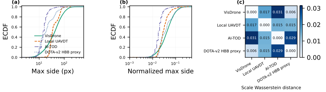
Fig. 1. Structural audit: (a) absolute horizontal-box support, (b) normalized support, and (c) equal-box-weight empirical 1-Wasserstein distances on normalized max side. DOTA-v2 is an axis-aligned horizontal-box (HBB) proxy derived from quadrilaterals and is structural-only; its distances are representation-conditioned rather than directly comparable to native horizontal-box sources.
