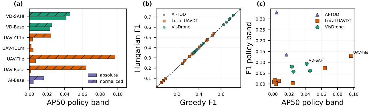
Fig. 2. Primary-grid rule and matching sensitivity: (a) AP_{50} bands over \Pi = \{\text{include-all, exclude/source-ignore-off, exclude/source-ignore-on}\} at the two headline scale rules (solid: absolute; hatched: normalized; VD=VisDrone, UAV=local UAVDT, AI=AI-TOD; Base=baseline, Tile=tiling, SAHI=slicing-aided inference, Y11n/Y11m=YOLO11 variants), (b) score-ordered greedy versus threshold-first Hungarian F_1 at confidence .25 and IoU .25/.50, and (c) AP_{50}/F_1 primary-grid policy-band relation. Circle/square/triangle markers denote VisDrone/local UAVDT/AI-TOD, respectively; points use source-consistent coverage.
