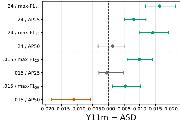
(b) Localization × metric control
