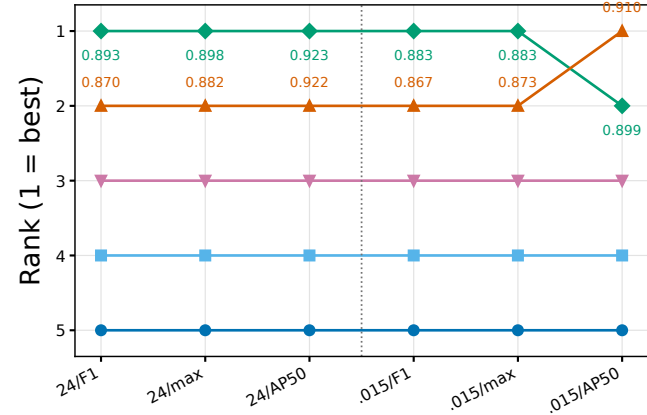
(a) Metric-conditioned ranks
