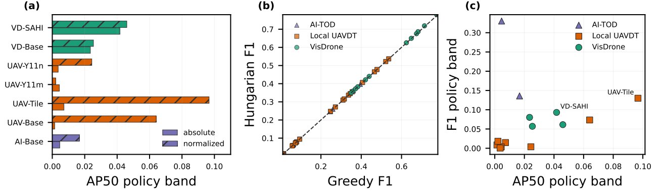
Fig. 2. Primary-grid rule and matching sensitivity: (a) AP_{50} bands over \Pi = \{include-all, exclude/source-ignore-off, exclude/source-ignore-on\} at the two headline scale rules (solid: absolute; hatched: normalized; VD=VisDrone, UAV=local UAVDT, AI=AI-TOD; Base=baseline, Tile=tiling, SAHI=slicing-aided inference, Y11n/Y11m=YOLO11 variants), (b) score-ordered greedy versus threshold-first Hungarian F_1 at confidence .25 and IoU .25/.50, and (c) AP_{50}/F_1 primary-grid policy-band relation. Circle/square/triangle markers denote VisDrone/local UAVDT/AI-TOD, respectively; points use source-consistent coverage.
