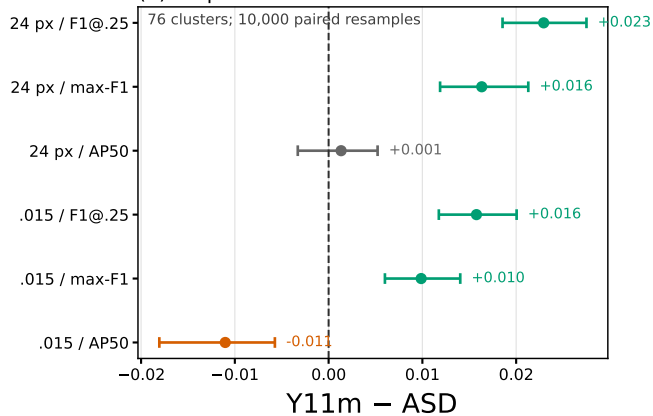
(b) Sequence-cluster 95% intervals
