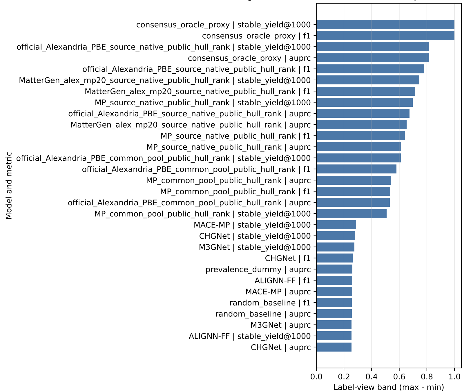
Fig. 1 Source-aware label views turn point estimates into bands
