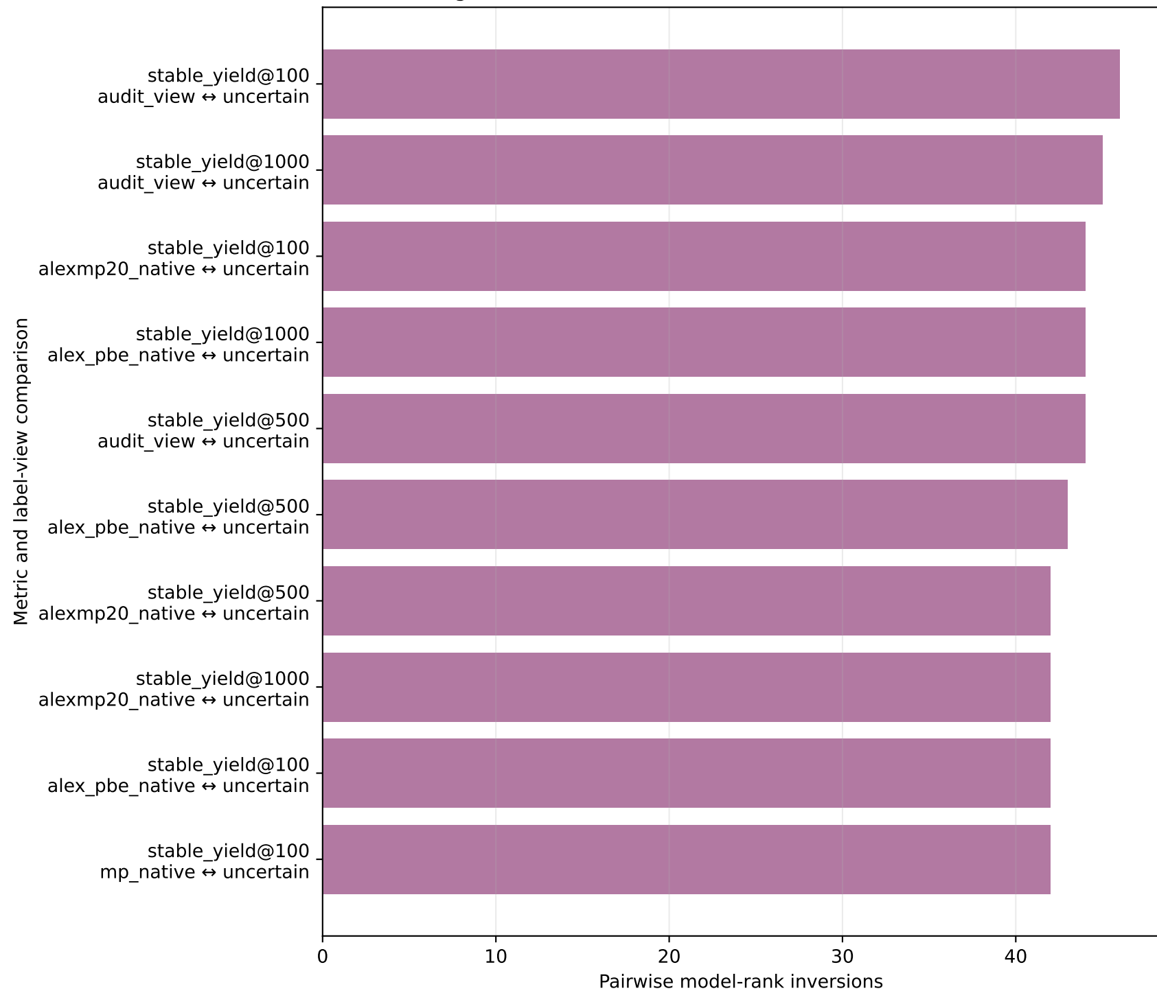
Fig. 3 Rank inversions across source-aware label views
