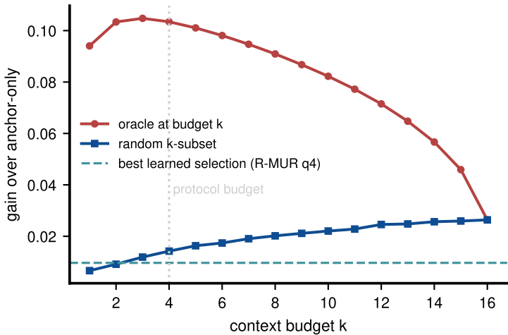
Perfect selection wants fewer contexts
