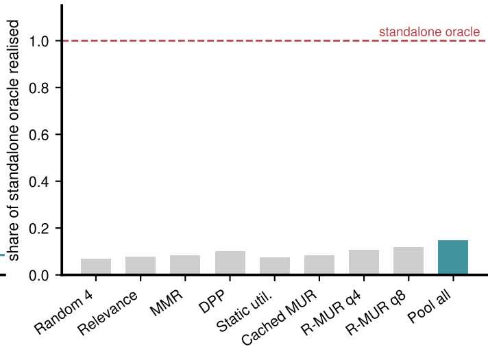
Every deployable policy is far below the oracle
