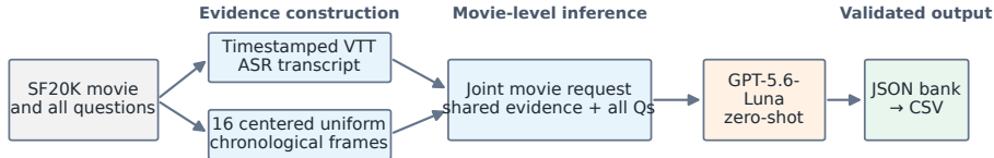
Figure 1. Movie-level joint inference. Timestamped ASR and centered uniform frames are paired with all questions from one film. The answerer emits one JSON bank, which is converted to the submission CSV.
