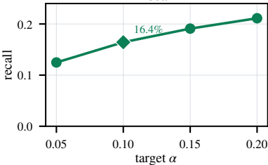
Recall
