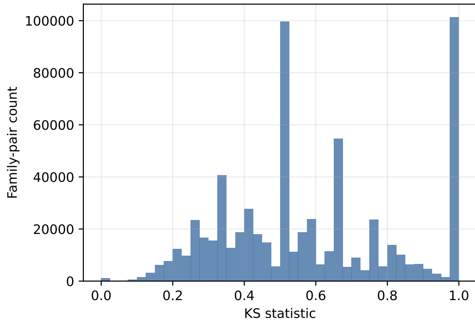
Two-sample KS, Bonferroni reject=0.000
