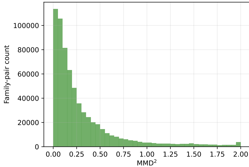
RBF MMD 2 , LOO mean=1.000
