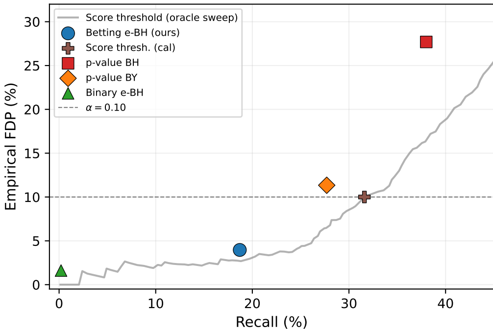
FDP-Recall Operating Points at \alpha = 0.10
