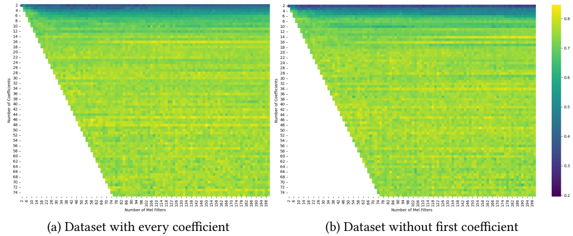
Figure 3: Neural Network F1 Score heatmaps for datasets with and without first coefficient
