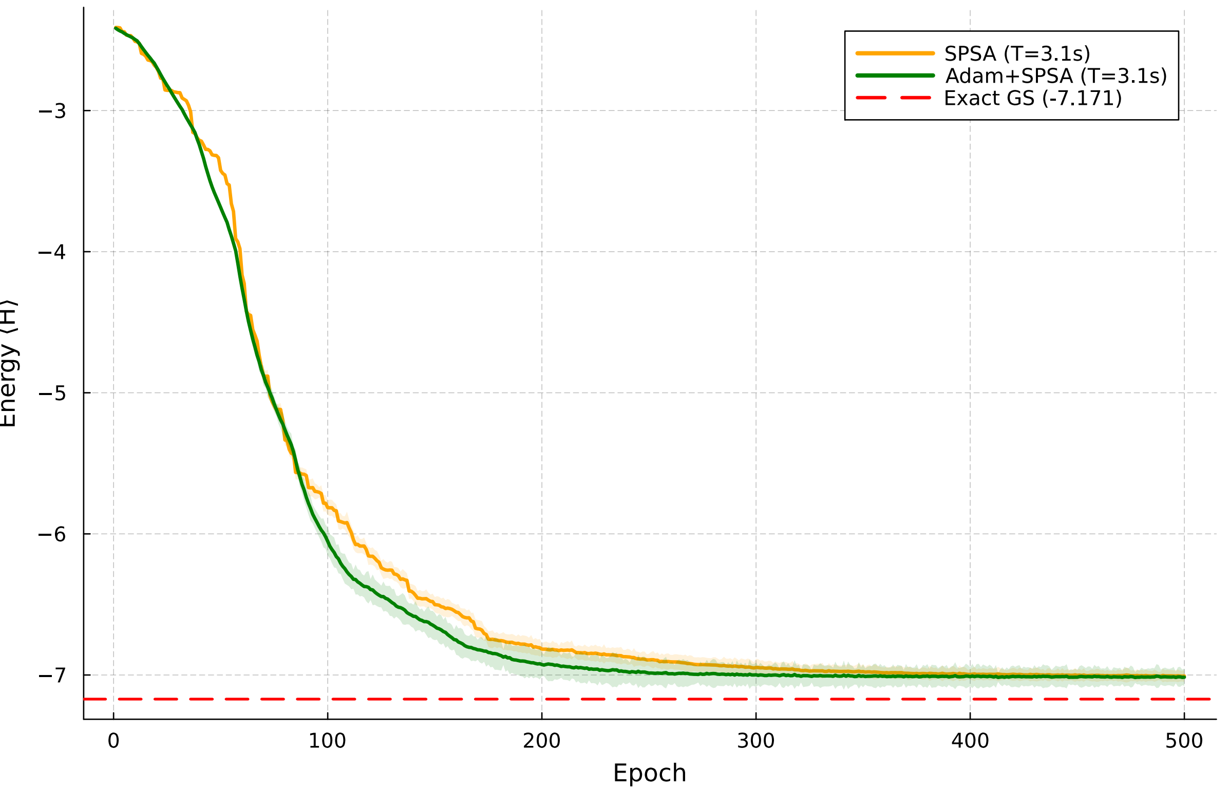
CPU MCWF (N=6, M=1000, HEA, L=1, N_θ=24, amplitude_damping, p=0.05)
