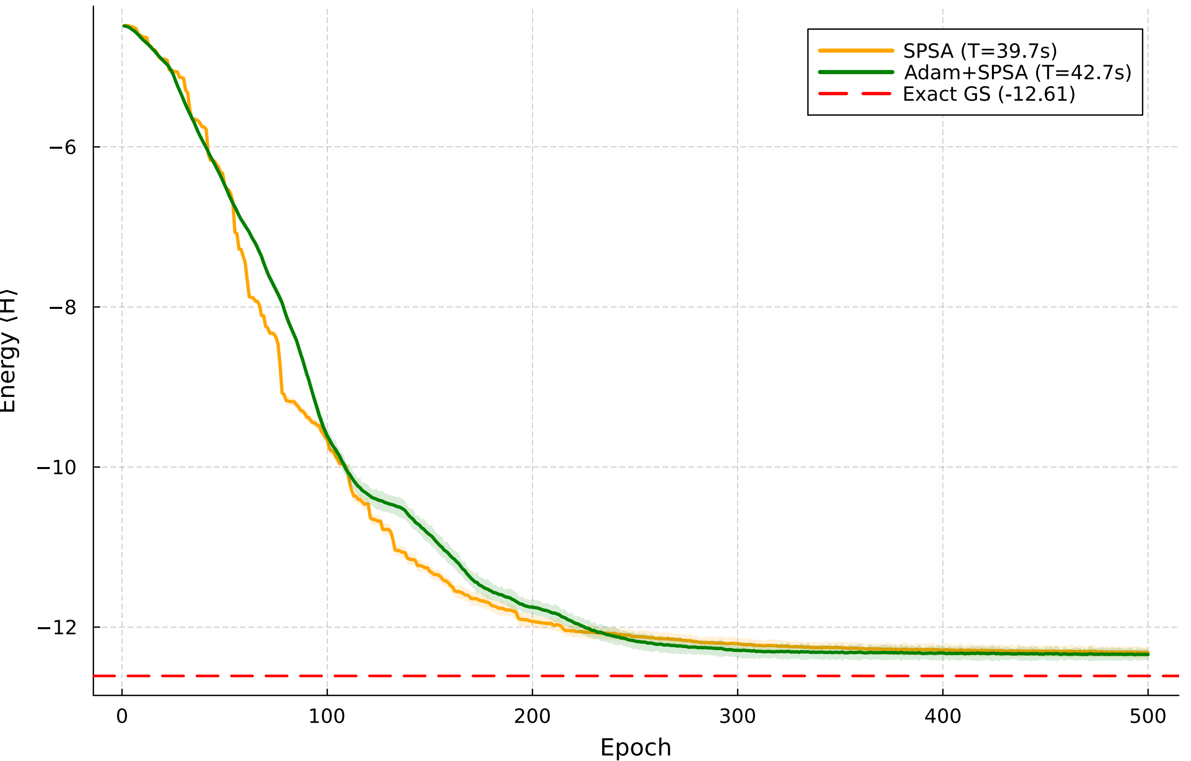
CPU MCWF (N=10, M=1000, HEA, L=1, N_θ=40, amplitude_damping, p=0.05)
