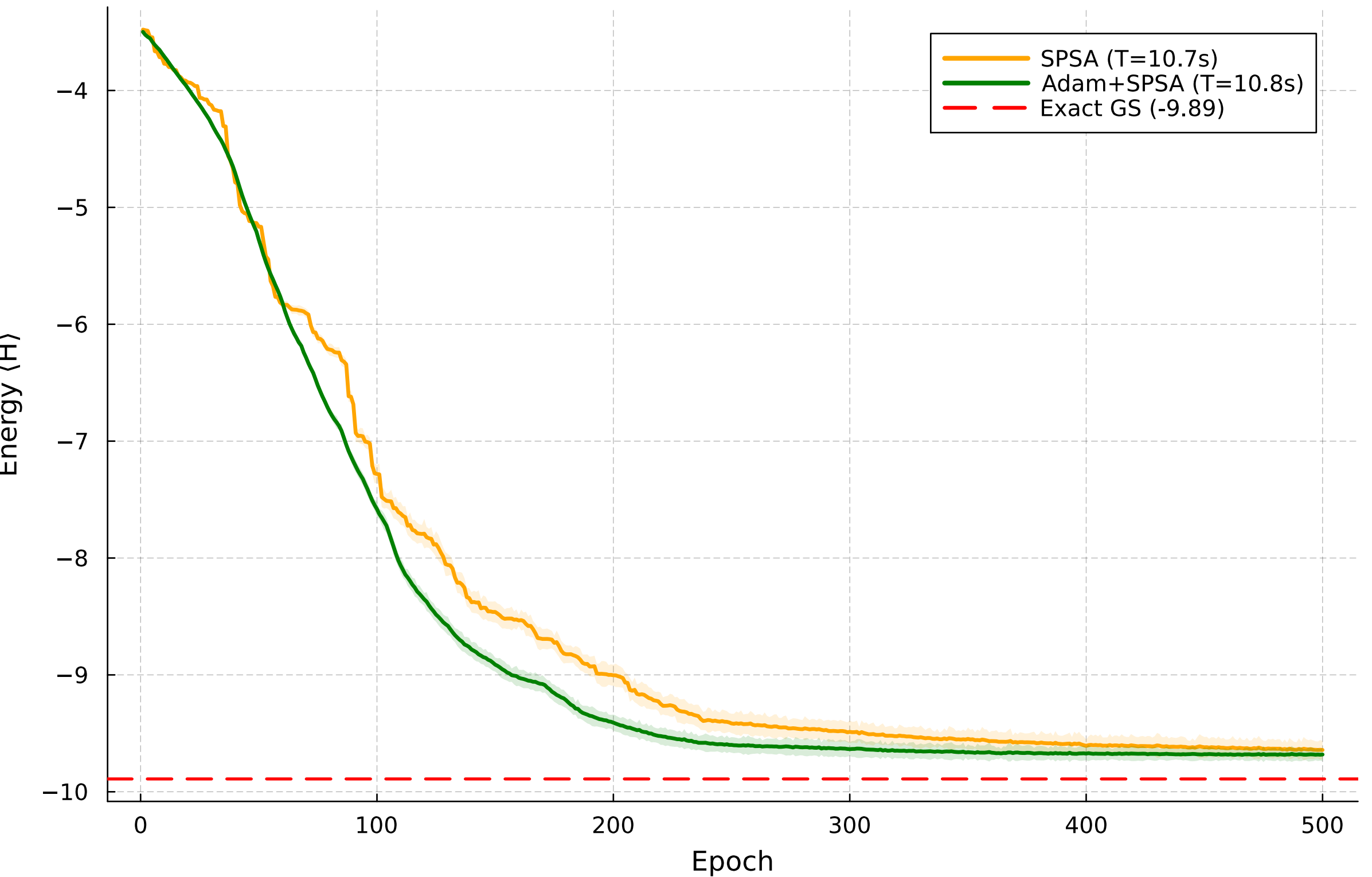
CPU MCWF (N=8, M=1000, HEA, L=1, N_θ=32, amplitude_damping, p=0.05)
