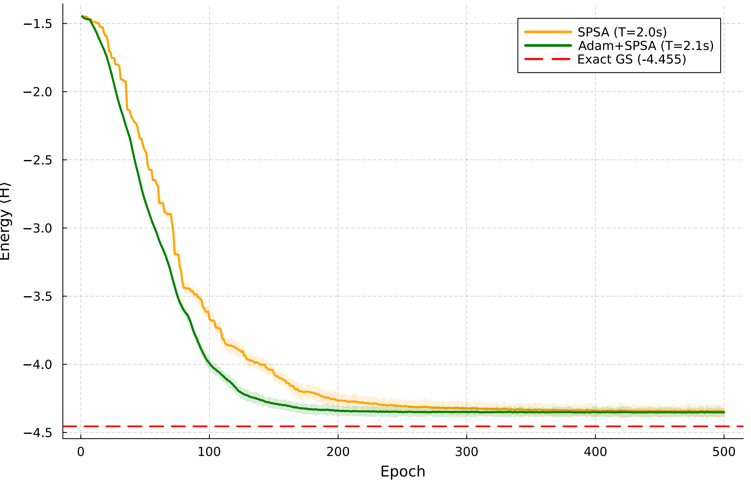
CPU MCWF (N=4, M=1000, HEA, L=1, N_θ=16, amplitude_damping, p=0.05)
