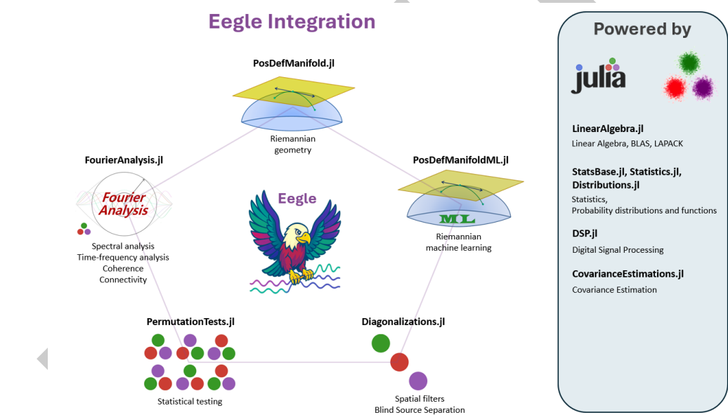
Figure 1: Julia package ecosystem currently integrated by Eegle.
