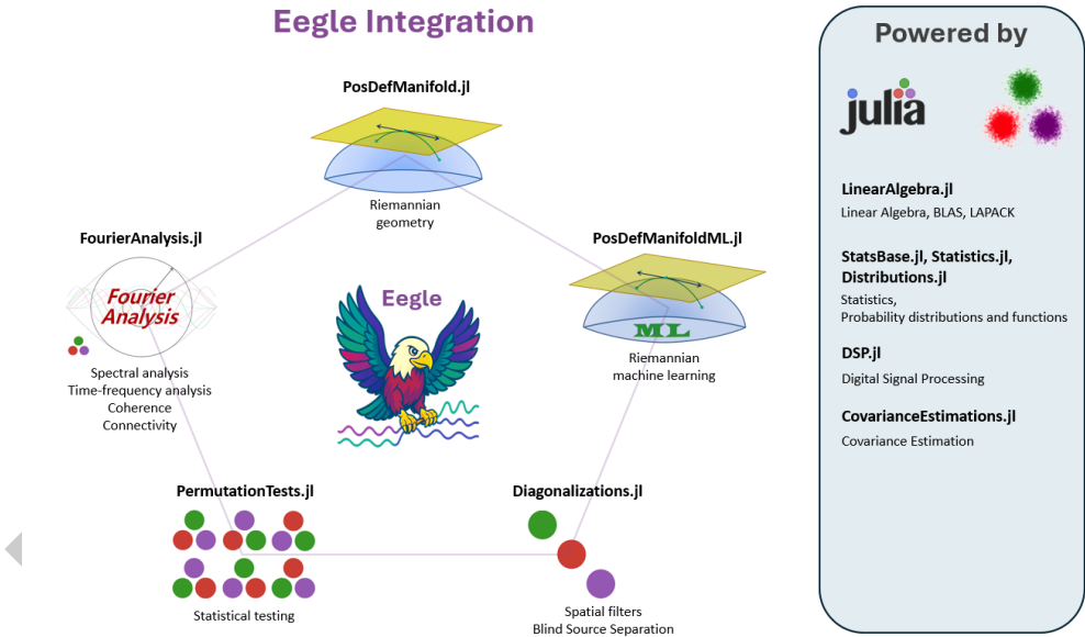
Figure 1: Julia package ecosystem currently integrated by Eegle.
