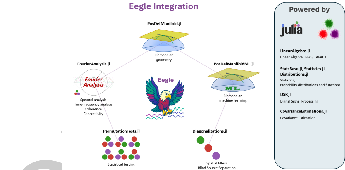
Figure 1: Julia package ecosystem currently integrated by Eegle .
