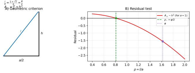
Fig. 2. Fibonacci-pyramid validation plot. Left: geometric cross-section with A_\Delta = \frac{al}{2} and h^2 = l^2 - (a/2)^2 . Right: residual A_\Delta - h^2 versus \rho = l/a , showing the zero at \rho = \frac{1+\sqrt{5}}{4} = \varphi/2 , while \rho = \varphi is non-zero.
