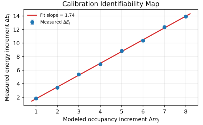
Fig. 6. Illustrative calibration map: measured energy increment versus modeled occupancy increment with uncertainty bars and fitted slope \mu c^2 .
