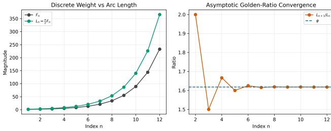
Fig. 2. Scaling consistency of the geometric model: left, Fibonacci weights and arc lengths L_n = \frac{\pi}{2} F_n ; right, convergence of L_{n+1}/L_n to the golden ratio \varphi .
