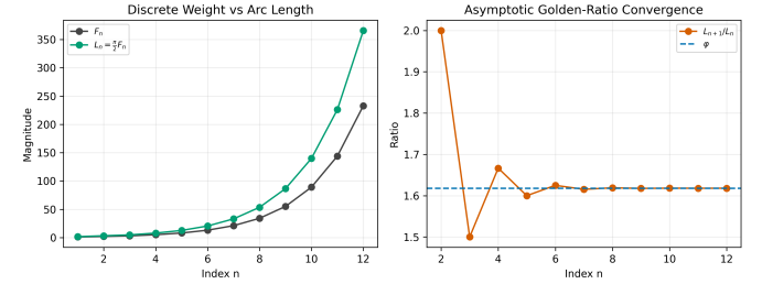
Fig. 5. Scaling consistency of the geometric model: Left, Fibonacci weights and arc lengths L_n = \frac{\pi}{2} F_n ; Right, convergence of L_{n+1}/L_n to the golden ratio \varphi .
