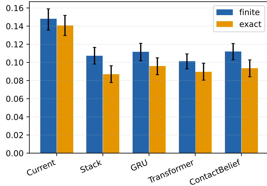
brier
