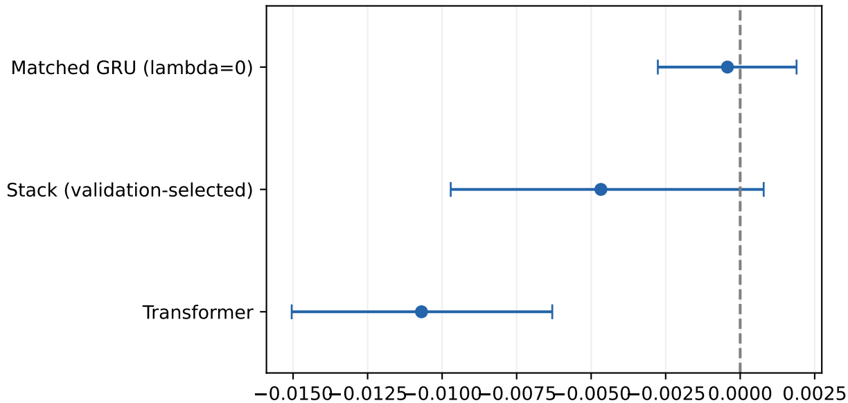
Brier improvement
