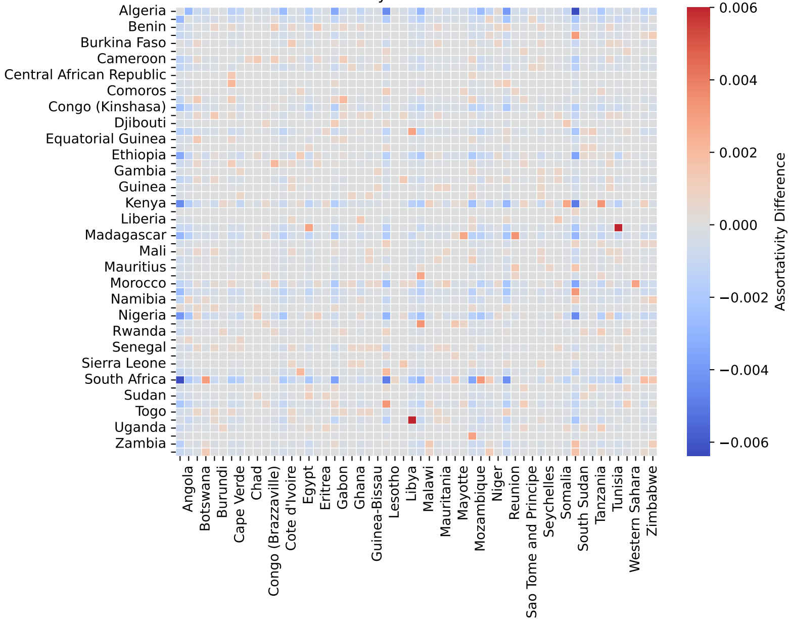
Assortativity Difference in Africa
