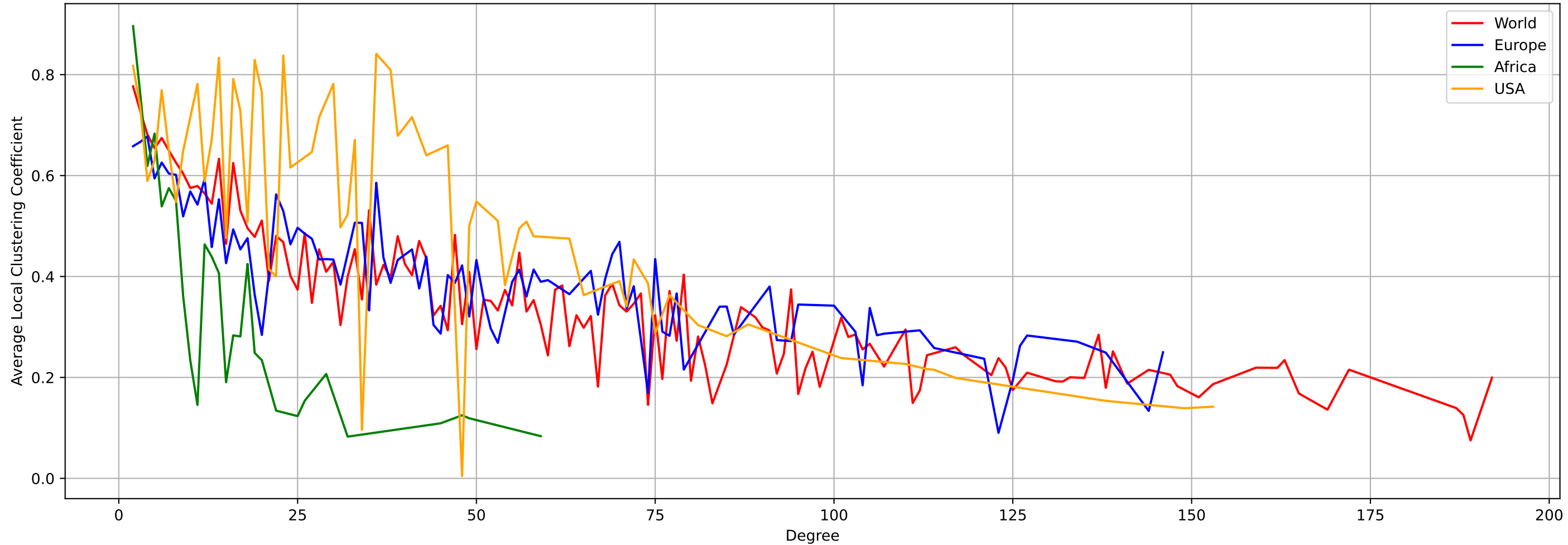
Average Local Clustering Coefficient for Nodes by Degree (deg <200)
