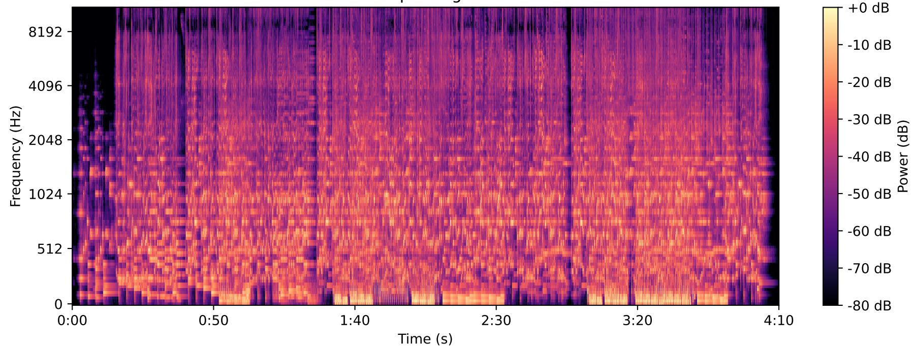
Mel-spectrogram
