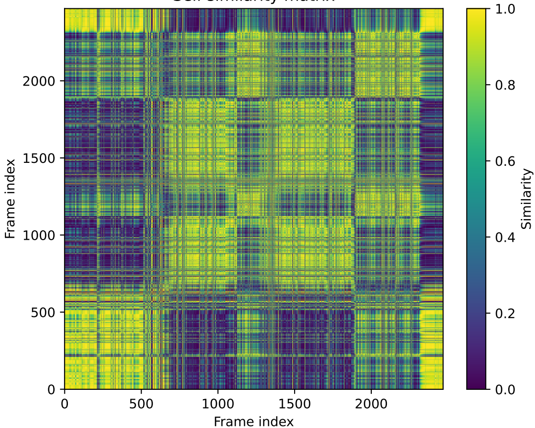
Self-similarity matrix
