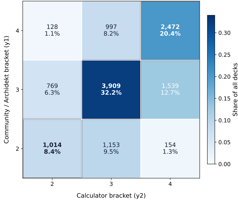
Figure 1: Agreement matrix between the community label y_{\text{arch}} and the calculator label y_{\text{calc}} on the 12,135-deck modeling set. Rows are ordered from bracket 4 to bracket 2. Each cell reports a count and its percentage of the full dataset. The diagonal contains exact matches; off-diagonal cells show disagreement direction. The calculator assigns a higher bracket than the author in 2,846 decks (23.5%) and a lower bracket in 1,894 decks (15.6%).
