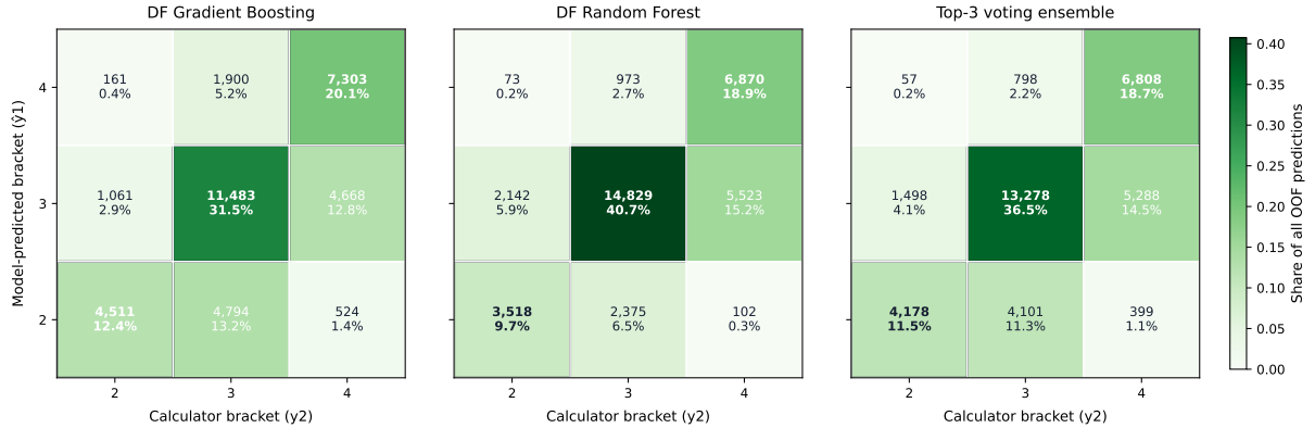
Figure 3: Agreement matrices between out-of-fold predictions \hat{y}_{\text{arch}} and the calculator label y_{\text{calc}} for the models highlighted in Table 7. Each cell reports a count and its percentage of all 36,405 OOF predictions. DF Gradient Boosting is the best individual community predictor and matches the calculator on 23,297 predictions (64.0%); its off-diagonal mass is 9,986 below the calculator (27.4%) and 3,122 above it (8.6%). DF Random Forest is the closest individual model to the calculator, with 25,217 exact matches (69.3%), 8,000 below-calculator errors (22.0%), and 3,188 above-calculator errors (8.8%). The top-3 voting ensemble is the best overall community predictor, with 24,264 exact matches (66.7%), 9,788 below-calculator errors (26.9%), and 2,353 above-calculator errors (6.5%).
