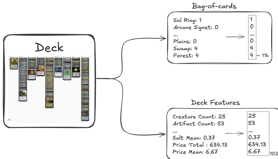
Figure 2: The two representations built from the same deck: Bag of Cards (sparse vector of card counts, \approx 11k dimensions) and Deck Features (dense vector of 102 structural attributes).
